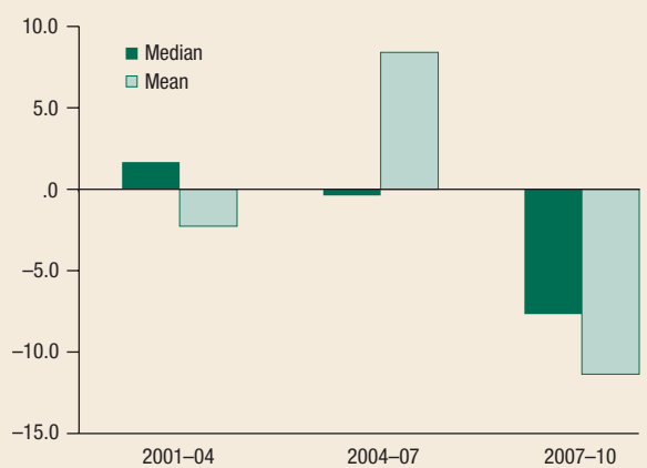
Figure 1. Change in median and mean incomes, 2001–10 SCF
